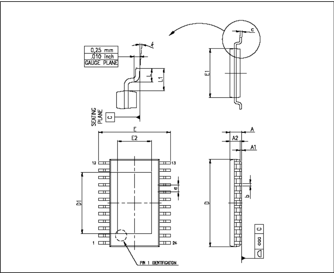
Figure 25. TSSOP24 Dimensions
