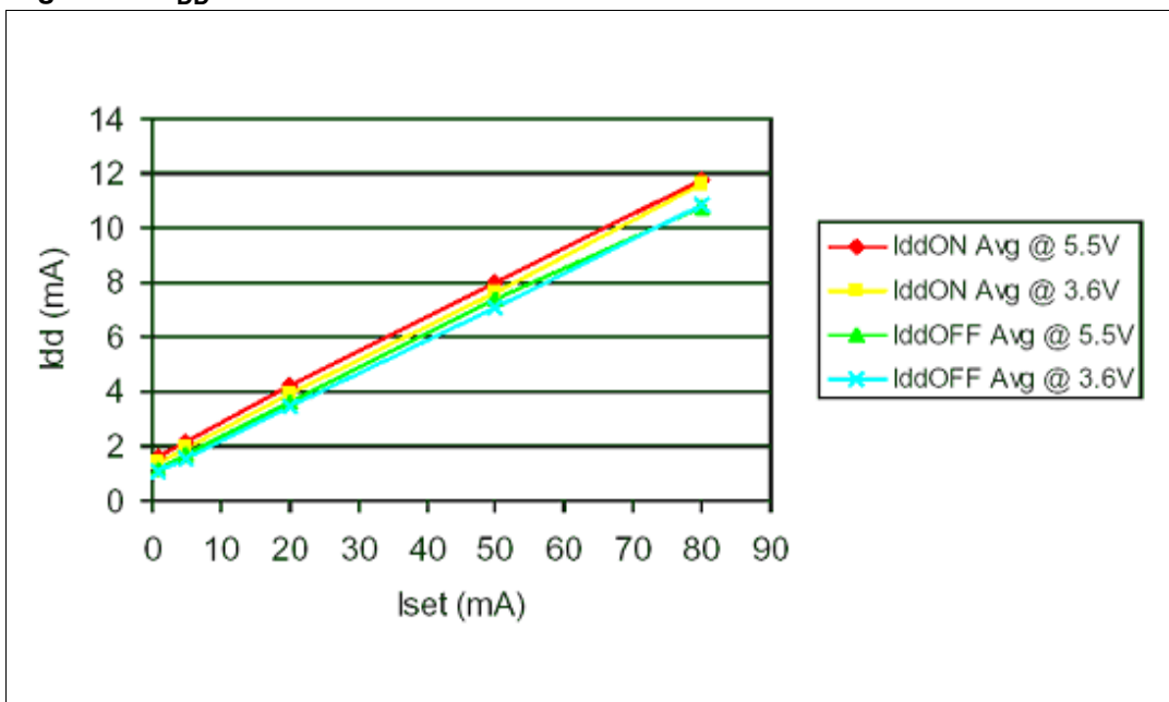
Figure 14. I_{DD} ON/OFF
