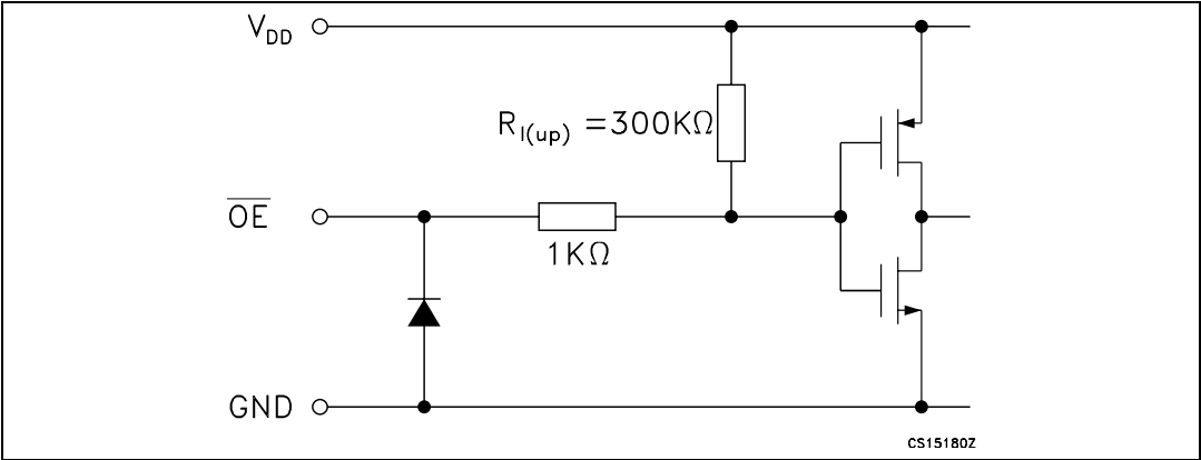
Figure 2. \overline{\text{OE}} Terminal
