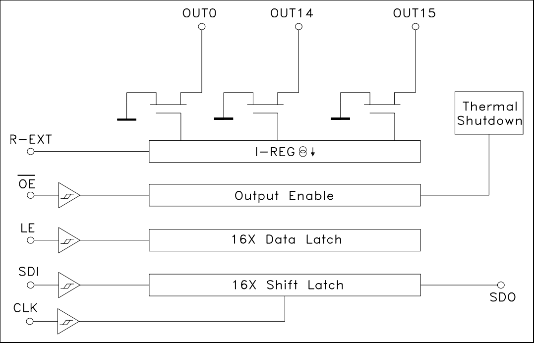
Figure 6. Block diagram
